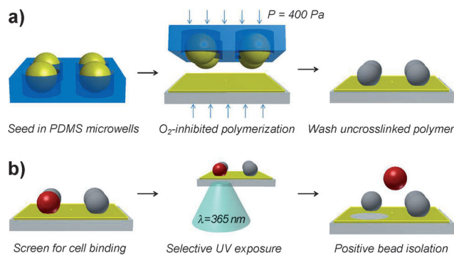
Scheme 1. Photogel preparation and process flow for patterning arrays of microbeads for selective bead retrieval. a) PEG-PS beads are swollen with photogel prepolymer, seeded into PDMS microwells, and transferred to a previously formed 15 \mu\text{m} -thick photogel layer on acrylated glass by \mu\text{TM} . Non-uniform polymerization allows uncrosslinked prepolymer to be washed from bead surfaces. b) Microbead arrays are screened for binding activity and positive beads are isolated by degrading photogel with 365 nm UV light.
